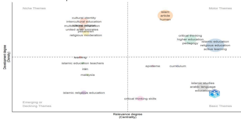
Gambar 21. Thematic Map .
