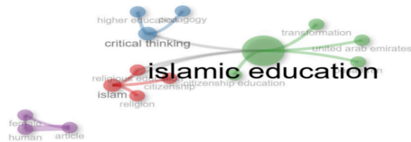
Gambar 20. Co-occurrence Network .
