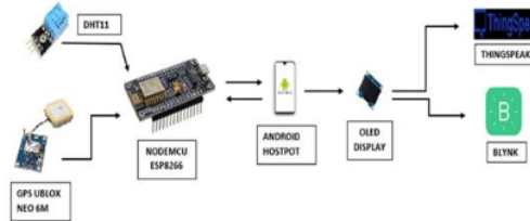
Fig 2. The general architecture of a telemetry system
