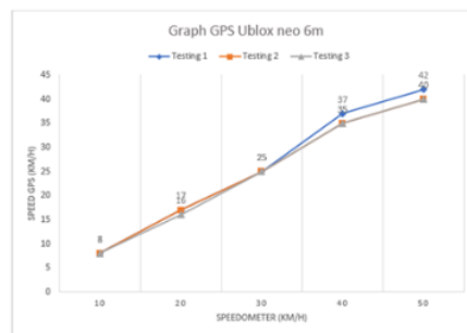
Graph 1. GPS U-blox Sensor Data
