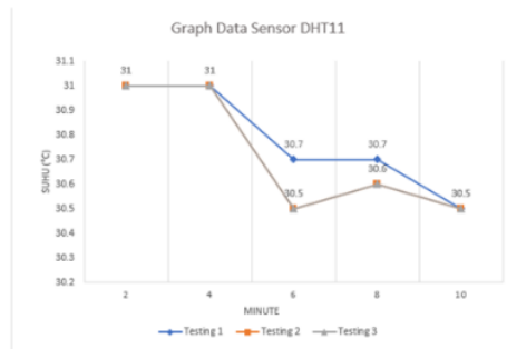
Graph 2. DHT 11 Sensor Data
