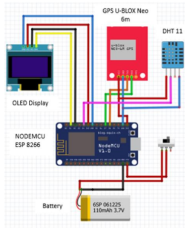
Fig 4. Hardware series
