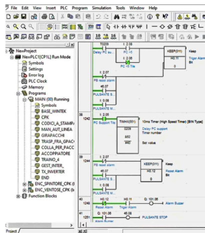
Gambar 5. Penambahan Program PLC
