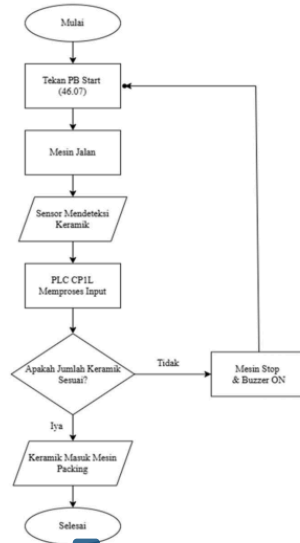
20 Gambar 3. Flowchart Sistem
