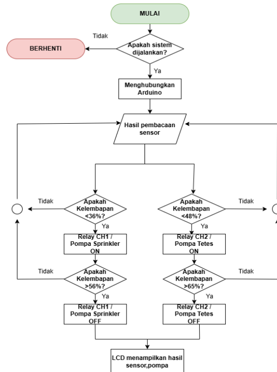
Gambar 2. Flowchart System
