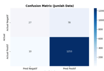
Gambar 5. Confusion Matrix Model Optimal
