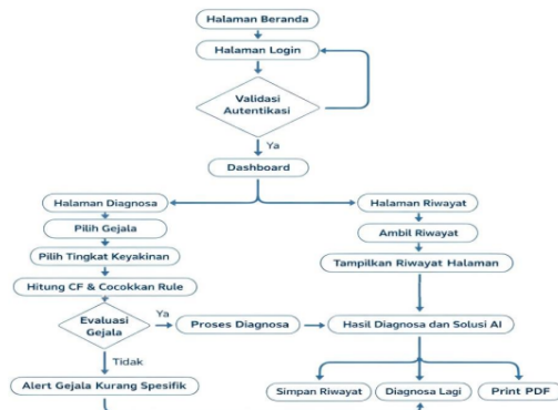
Gambar 2. Flowchart User
