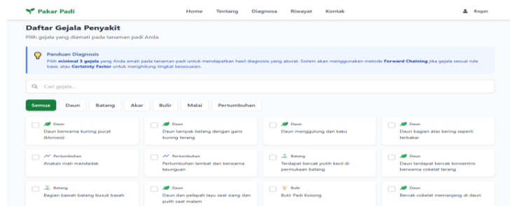
Gambar 7. Halaman Diagnosa
