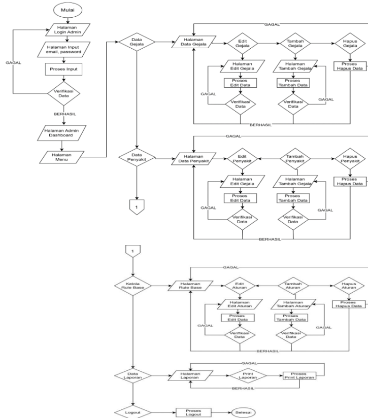
Gambar 3. Flowchart Admin
