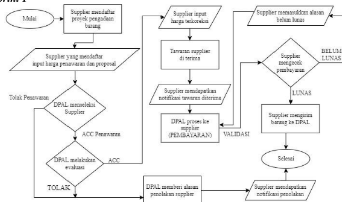
Gambar 2. Flowchart E-Procurement
