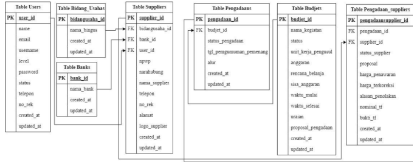
Gambar 3. Database E-Procurement
