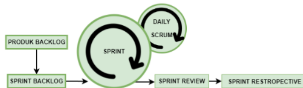
Gambar 1. Metode Scrum
