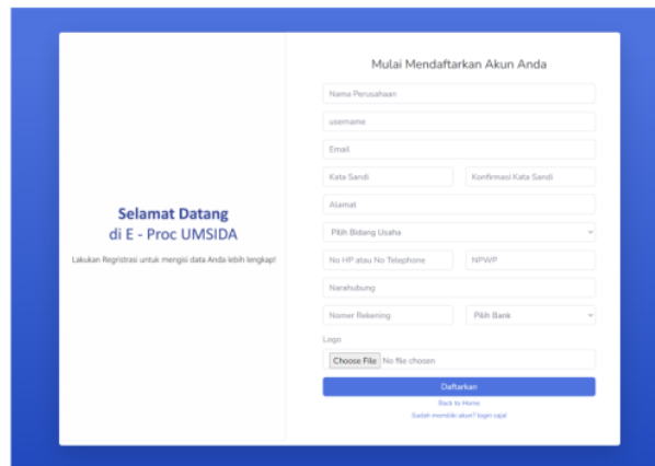
Gambar 5. Halaman Register
