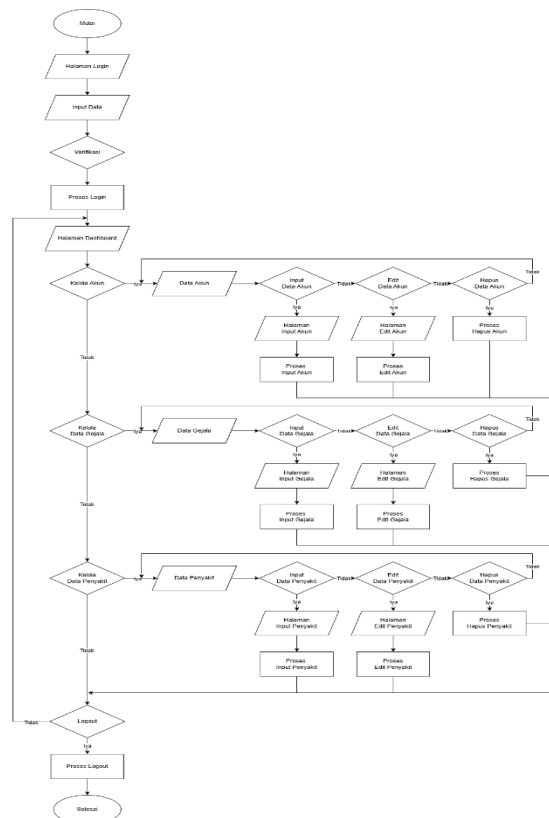
Gambar 2.3 Flowchart Admin
