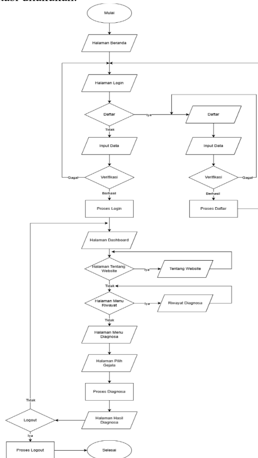
Gambar 2.2 Flowchart User
