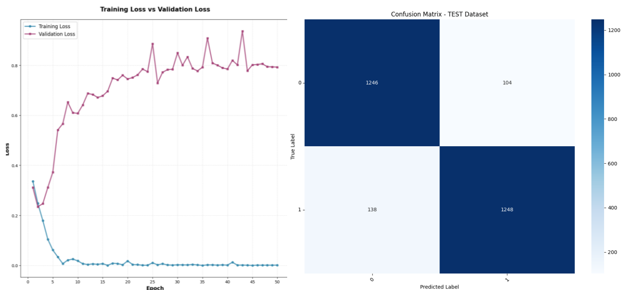
Gambar 5. Training, Validation Loss dan Confusion Matrix Skenario Ketiga
