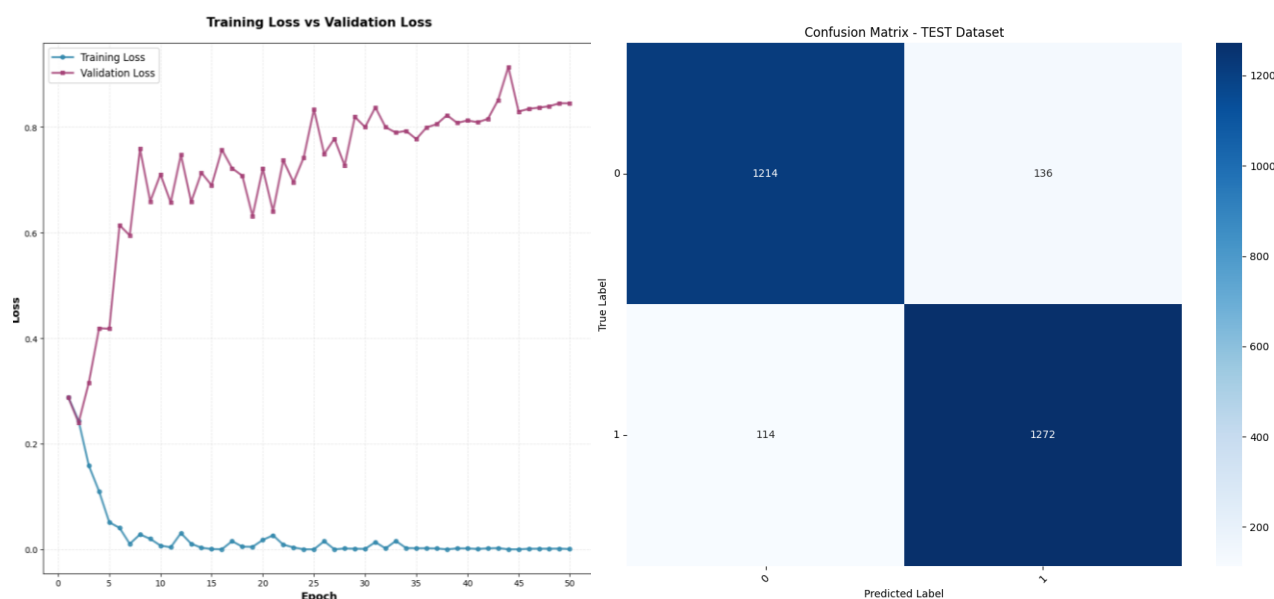
Gambar 3. Training, Validation Loss dan Confusion Matrix Skenario Pertama
