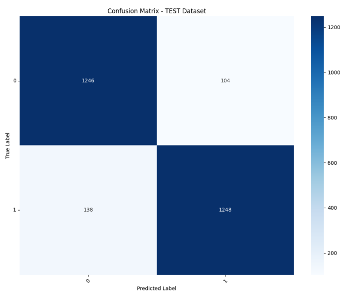
Gambar 6. Confusion Matrix IndoBERTtweet + BiLSTM
